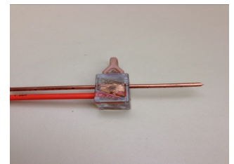
TS6B-19-C: 6 AWG Bare Ground to TRACE-SAFE
